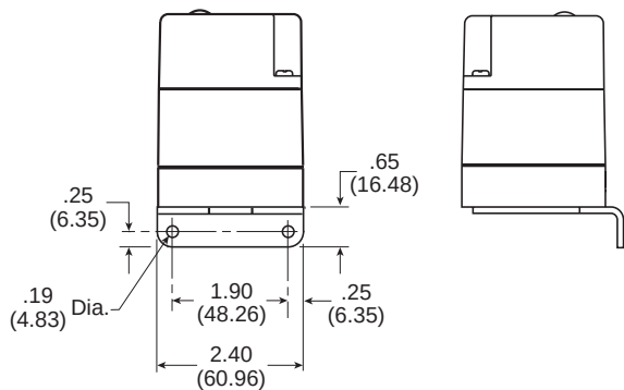
Angled Bracket
