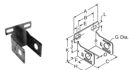
C-Bracket GPA-97-010
