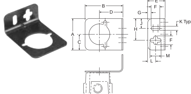
L-Bracket PS419
