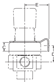
L-Bracket PS417B (Includes Panel Mount Nut)
