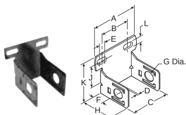
C-Bracket GPA-97-010
