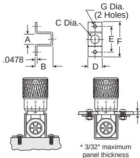
Mounting Bracket
