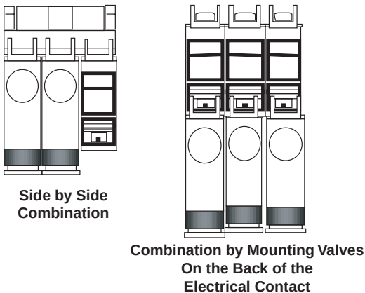
Electrical Contacts and Valves can be Combined Either Side by Side, or by Mounting the Valve on the Back of the Electrical Contact.
