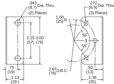
Mounting Bracket: 446-707-025
