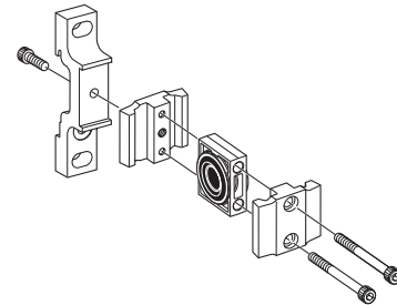
T-Bracket with Joiner Set GPA-96-312
