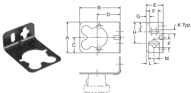
L-Bracket PS417B
