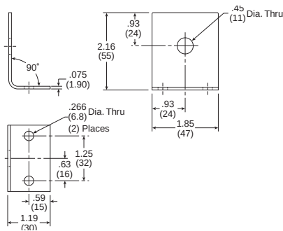
Mounting Bracket: 446-707-045
