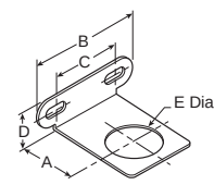
L-Bracket GRP-96-739
