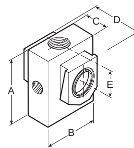
Modular Manifold Block (3 Auxiliary Ports) GPA-95-919
